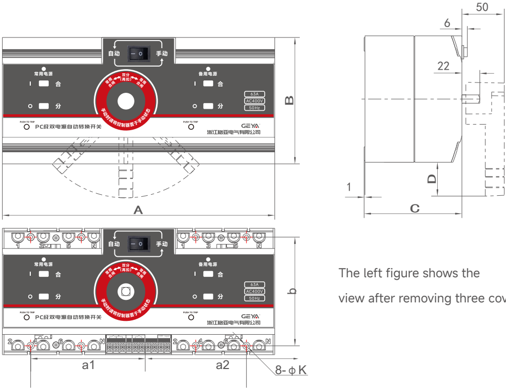
Installation dimensions of integral dual power supply automatic transfer switch
